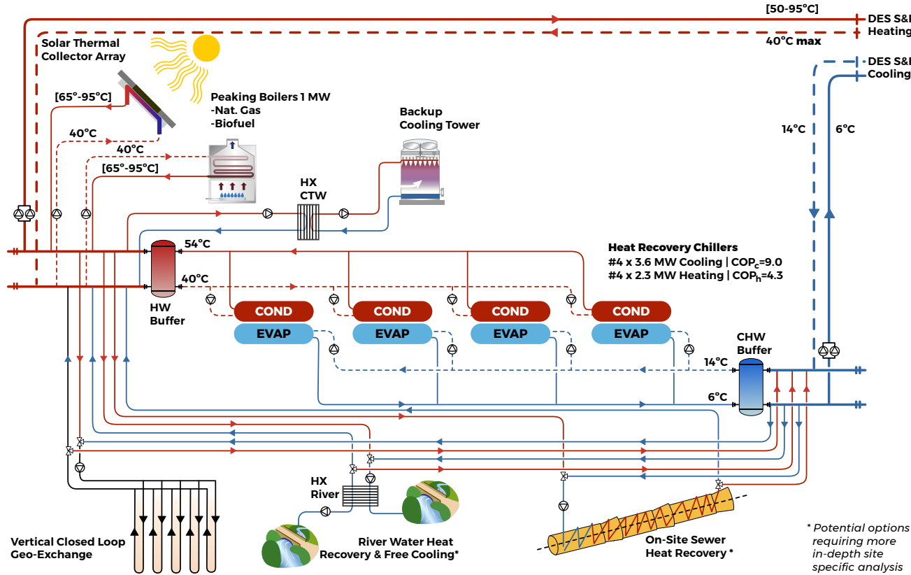
Figure 3. District geoechange system.
